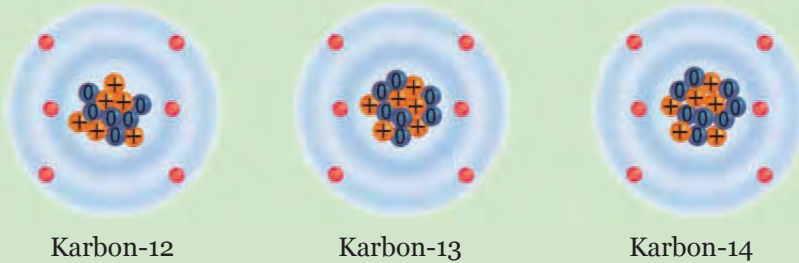
Gambar 4.14 Isotop-Isotop Atom Karbon
