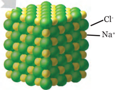
Gambar 4.18 Kristal Natrium Klorida (Garam Dapur)
