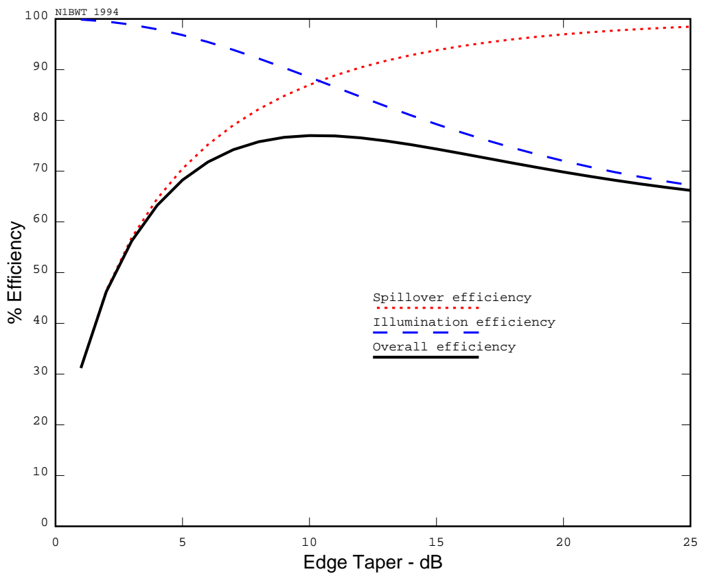
Figure 4-7. Efficiency vs. Edge Taper for a Dish
