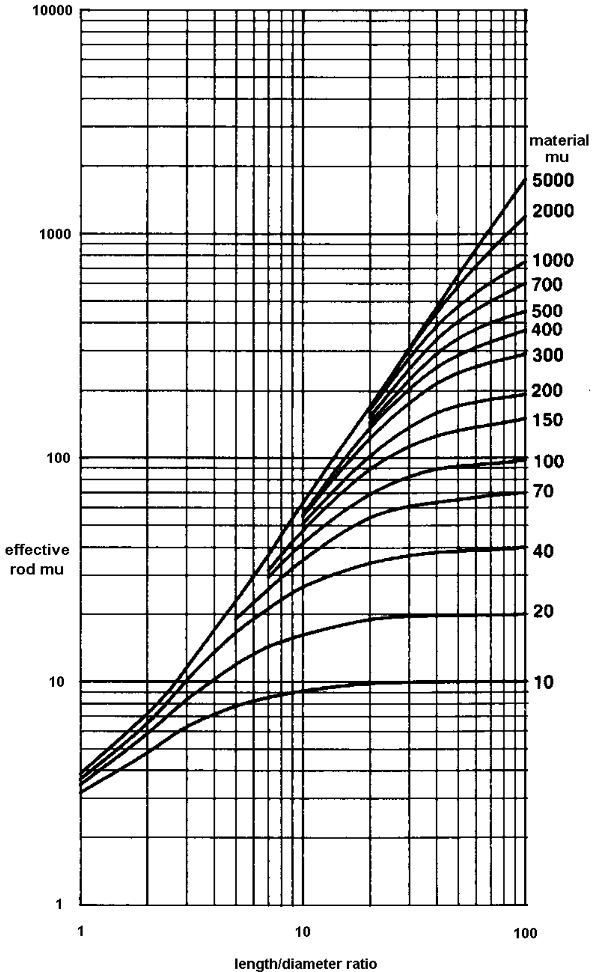
Effective Rod Permeability versus length/diameter Ratio
